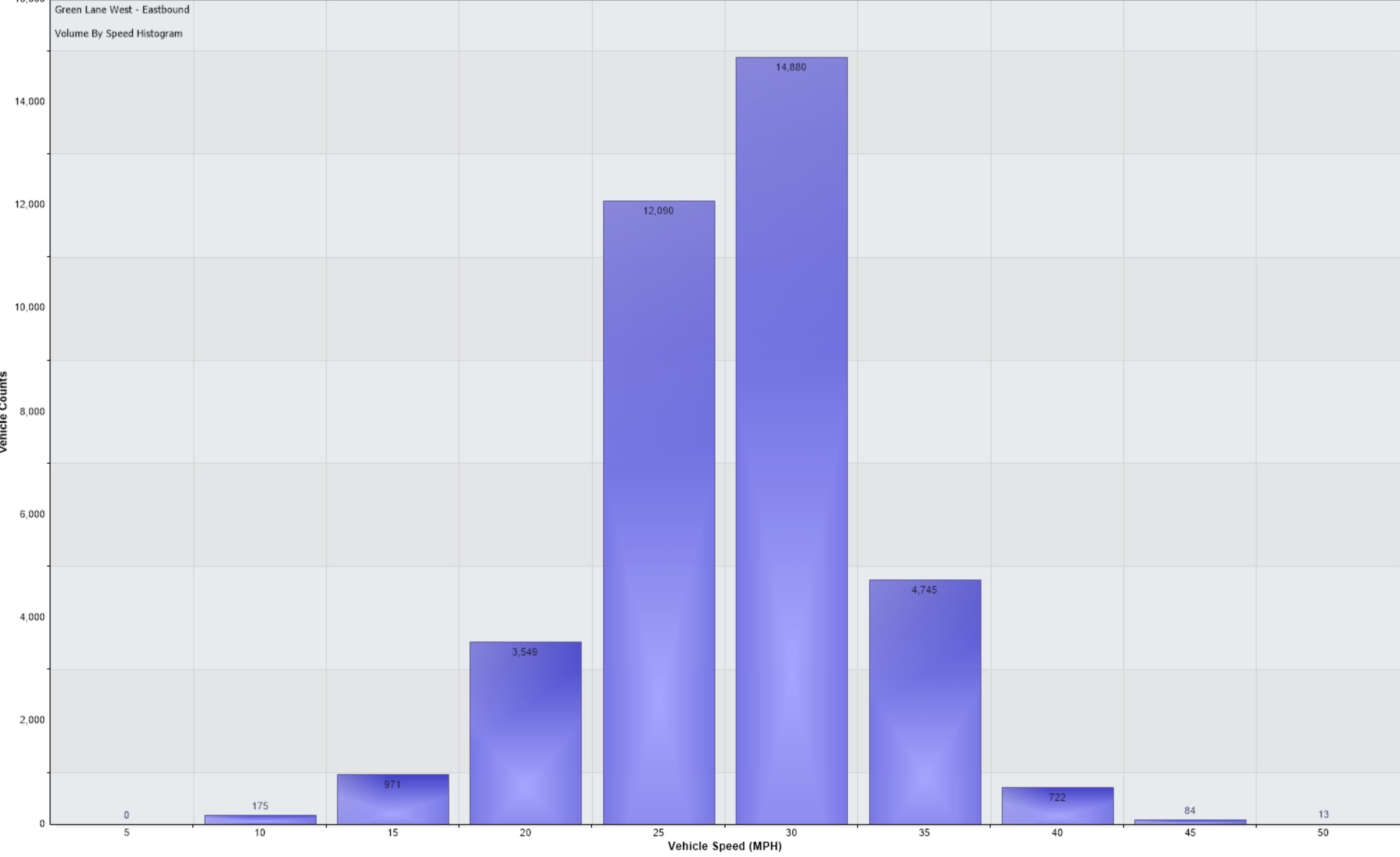
Vehicle Counts Vs. Speed [Green Lane West - Eastbound: Incoming]
