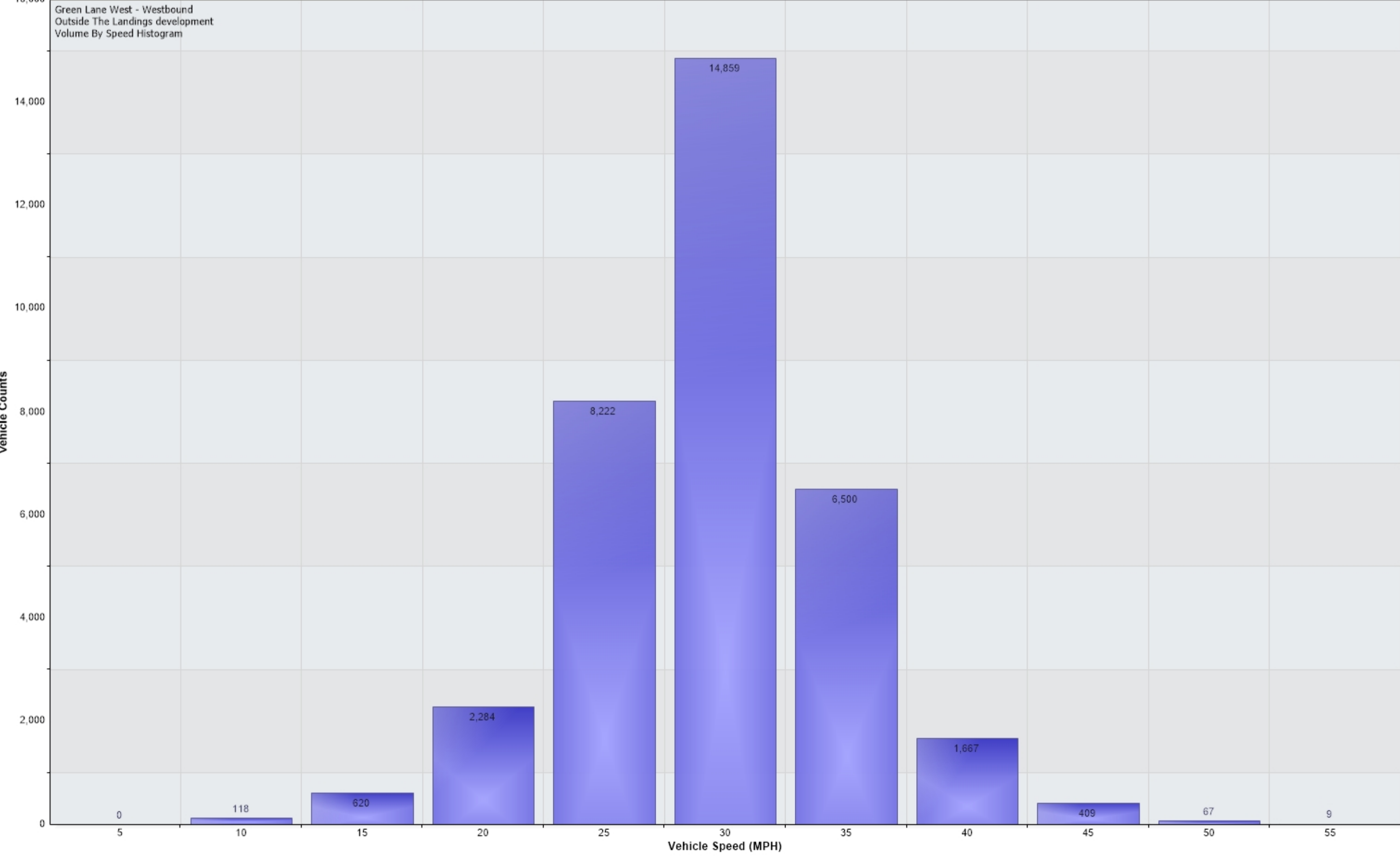
Vehicle Counts Vs. Speed [Green Lane West - Westbound: Incoming]
